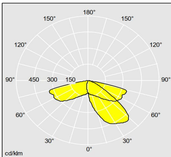
Figure 3-4 – Luminaire Distribution
