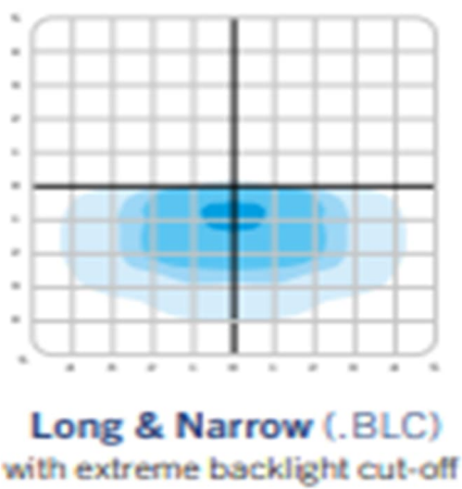
Figure 3-2 – Luminaire Distribution
